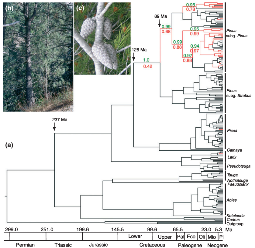
Fig. 2 Ancestral state reconstruction for canopy seed storage (serotiny). (a) Green values are the posterior probability of phylogenetic certainty at the corresponding node. Red values are the posterior probability of the reconstructed state at the corresponding node. Red lines represent evolutionary pathways (extant species/internal node/stem) for serotiny. Ma, million years ago. Pal, Paleocene; Eco, Eocene; Oli, Oligocene; Mio, Miocene; Pl, Pliocene. (b) Serotinous Pinus attenuata , showing retention of dead branches on its ~ 20 cm thick trunk. (c) Five-year-old serotinous cones, 12 cm long, of Pinus halepensis .
