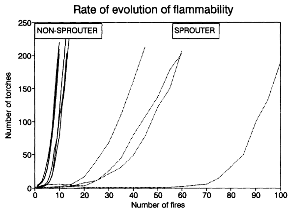
Fig. 2. Simulated dynamics of invasion of a flammable mutant into a non-flammable population. Solid lines indicate the population growth of non-sprouters and dashed lines of sprouters. Several simulation runs are shown to indicate the variance in rates of spread.
